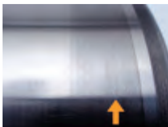
Figure 2 Adhesion occurs in equipment operating in the mixed and boundary lubrication regimes due to insufficient lube supply, inadequate viscosity, incorrect internal clearances, incorrect installation or misalignment.
