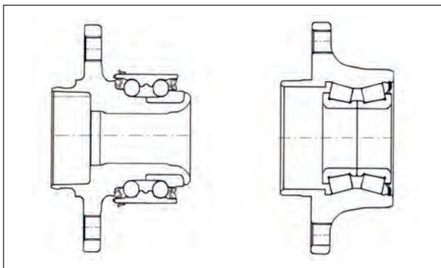
Picture 5 CRB2 & CRT2
