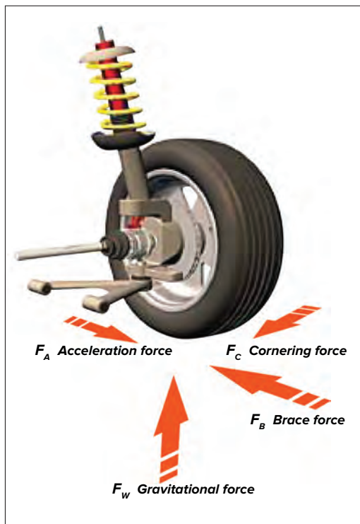
Picture 1 Wheel affecting forces
